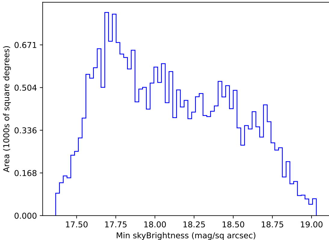
ddf_acor_sf10_ls20_lsr10_v3.4_10yrs All sky i band: Min skyBrightness
