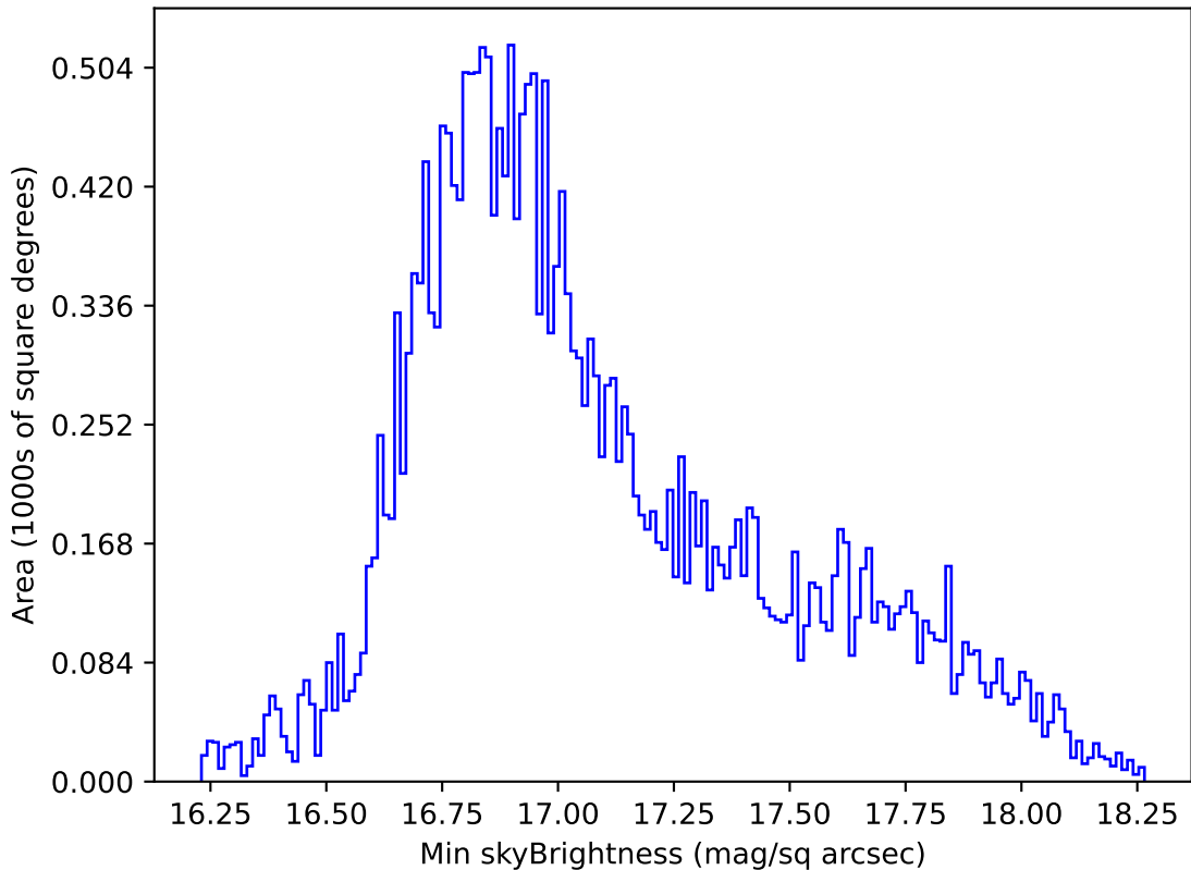
ddf_acor_sf10_lsf20_lsr10_v3.4_10yrs All sky all bands: Min skyBrightness
