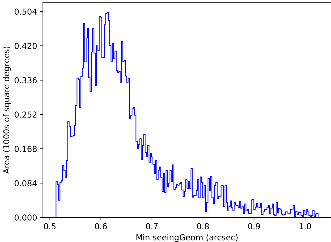
ddf_acor_sf10_lsf20_lsr10_v3.4_10yrs Yr 1 z band: Min seeingGeom
