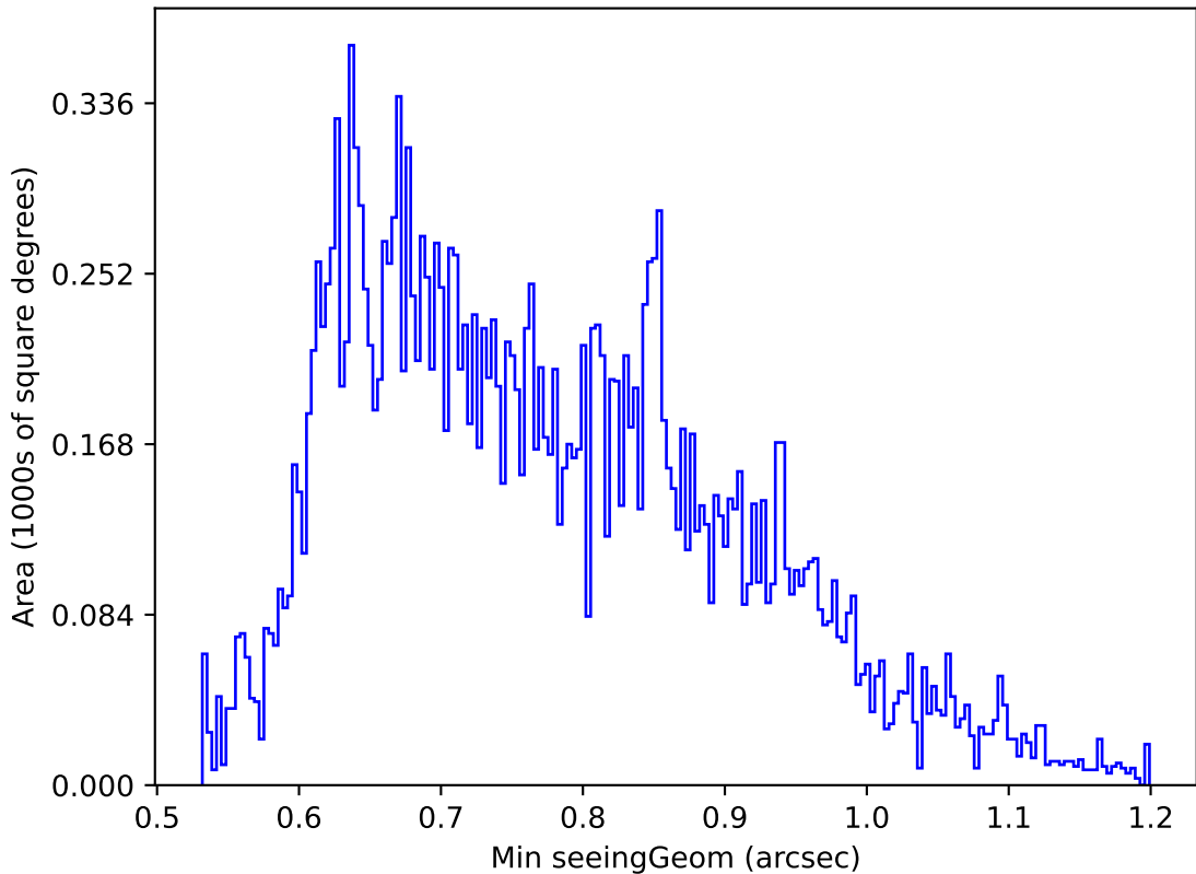
ddf_acor_sf10_lsf20_lsr10_v3.4_10yrs Yr 1 u band: Min seeingGeom
