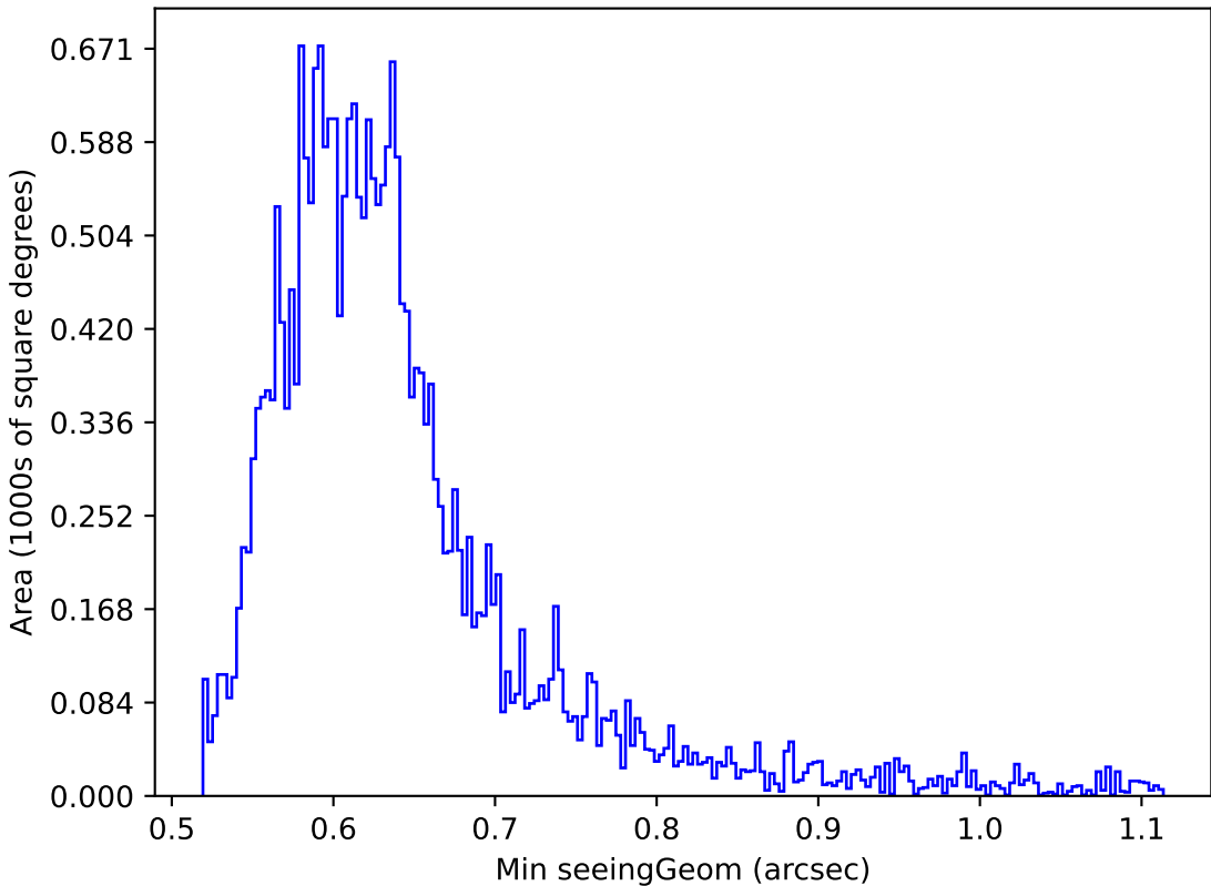
ddf_acor_sf10_ls20_lsr10_v3.4_10yrs Yr 1 r band: Min seeingGeom
