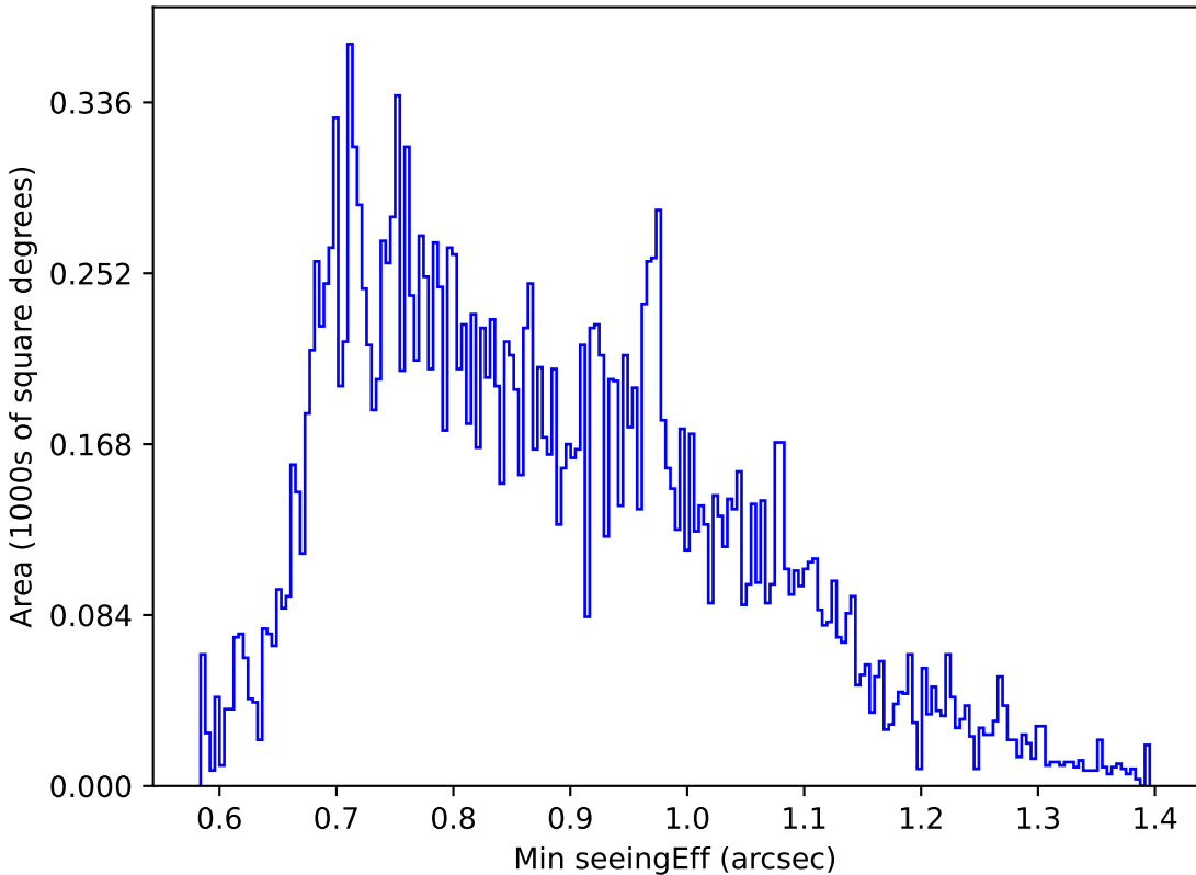
ddf_acor_sf10_lsf20_lsr10_v3.4_10yrs Yr 1 u band: Min seeingEff
