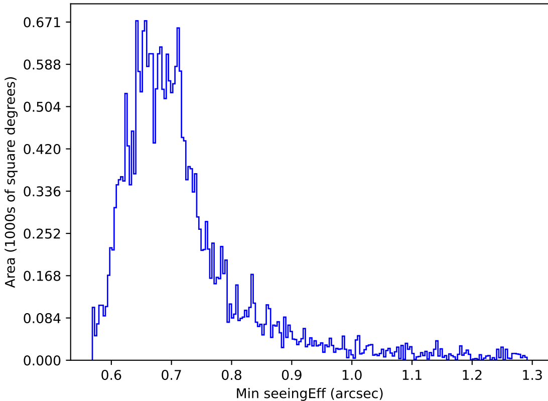
ddf_acor_sf10_lsf20_lsr10_v3.4_10yrs Yr 1 r band: Min seeingEff
