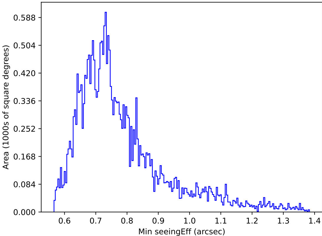
ddf_acor_sf10_lsf20_lsr10_v3.4_10yrs Yr 1 g band: Min seeingEff
