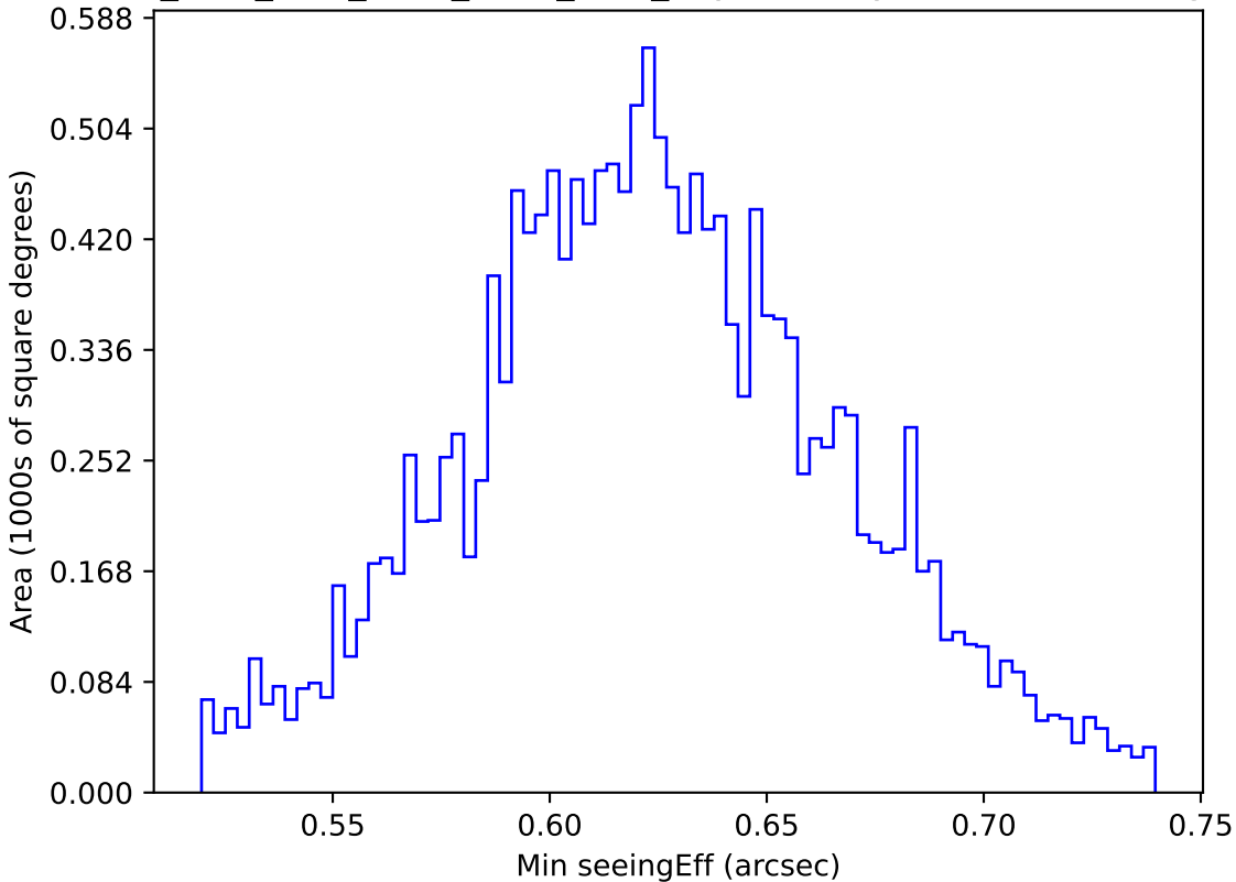
ddf_acor_sf10_lsf20_lsr10_v3.4_10yrs WFD y band: Min seeingEff
