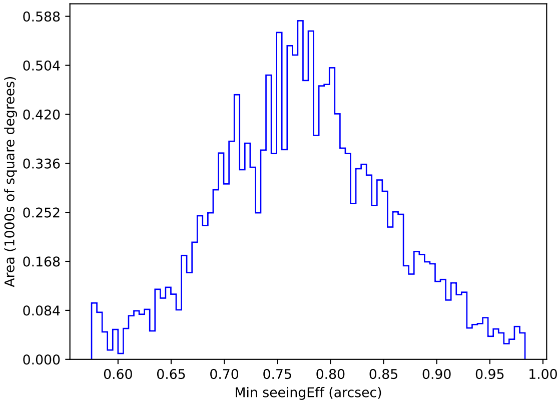
ddf_acor_sf10_lsf20_lsr10_v3.4_10yrs WFD u band: Min seeingEff
