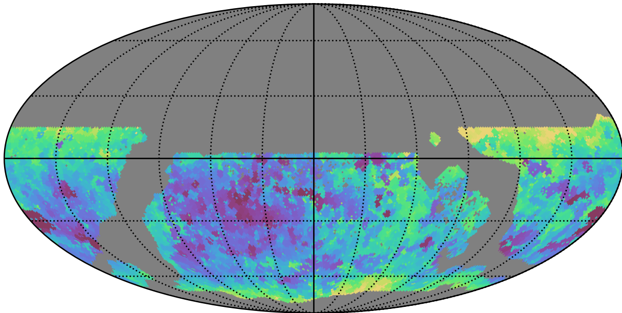
ddf_acor_sf10_lsf20_lsr10_v3.4_10yrs WFD r band: Min seeingEff
