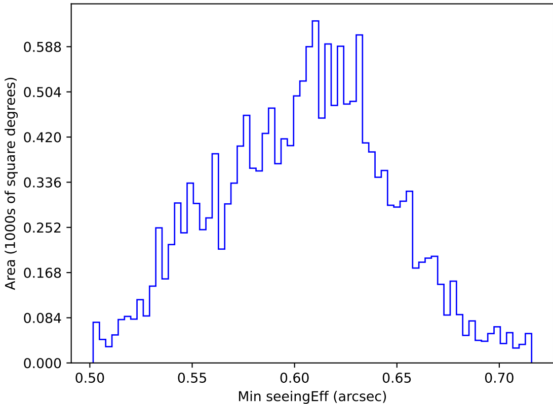
ddf_acor_sf10_lsf20_lsr10_v3.4_10yrs WFD i band: Min seeingEff
