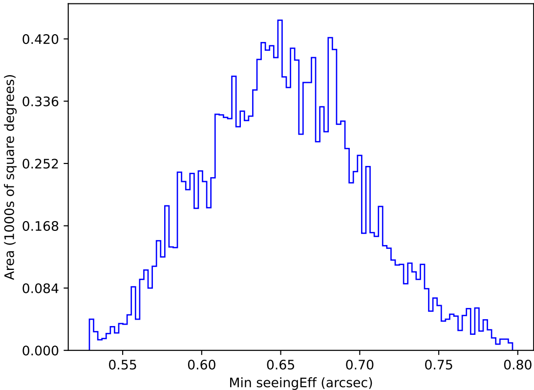
ddf_acor_sf10_lsf20_lsr10_v3.4_10yrs WFD g band: Min seeingEff
