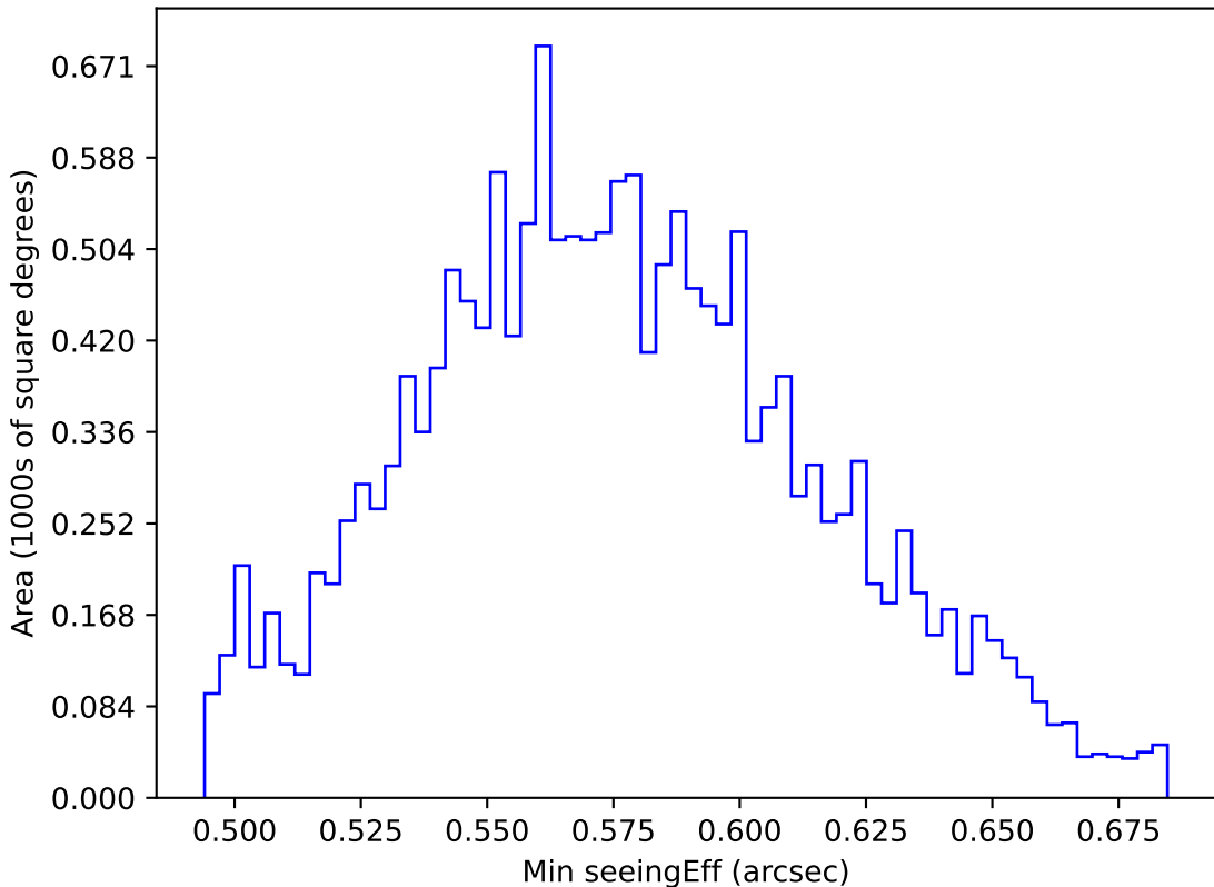
ddf_acor_sf10_lsf20_lsr10_v3.4_10yrs WFD all bands: Min seeingEff
