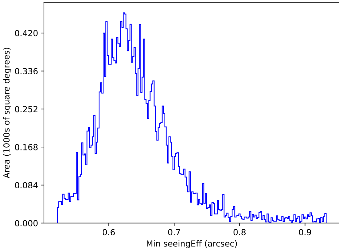
ddf_acor_sf10_lsf20_lsr10_v3.4_10yrs All sky y band: Min seeingEff
