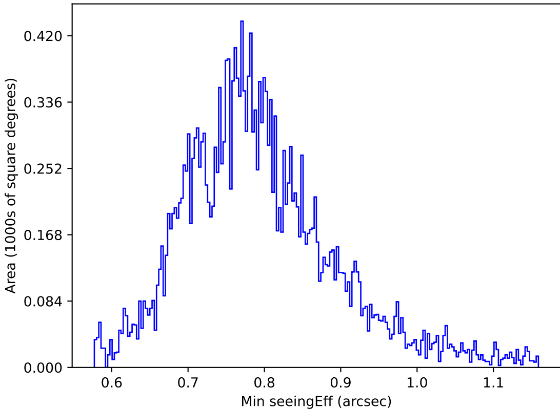
ddf_acor_sf10_lsf20_lsr10_v3.4_10yrs All sky u band: Min seeingEff
