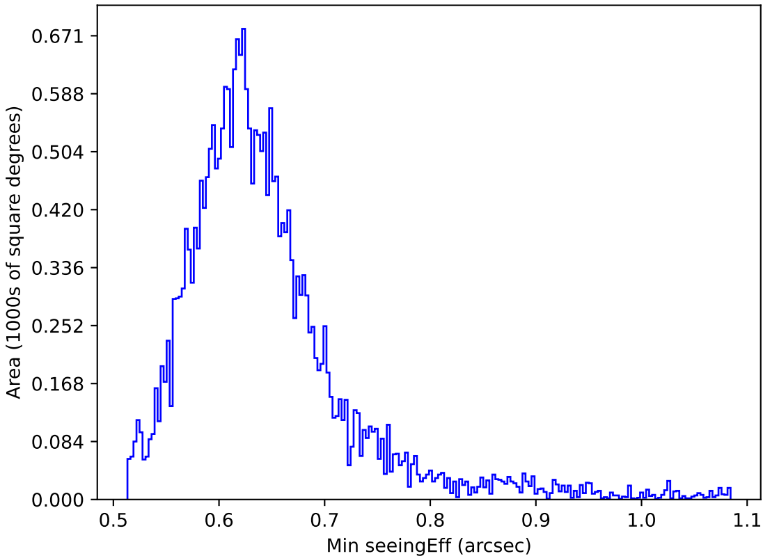
ddf_acor_sf10_lsf20_lsr10_v3.4_10yrs All sky r band: Min seeingEff
