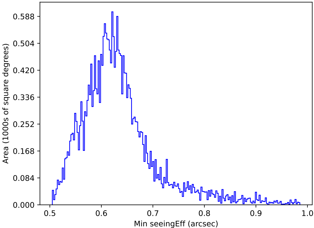
ddf_acor_sf10_lsf20_lsr10_v3.4_10yrs All sky i band: Min seeingEff
