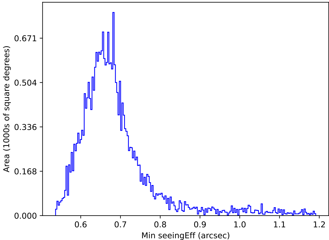
ddf_acor_sf10_lsf20_lsr10_v3.4_10yrs All sky g band: Min seeingEff
