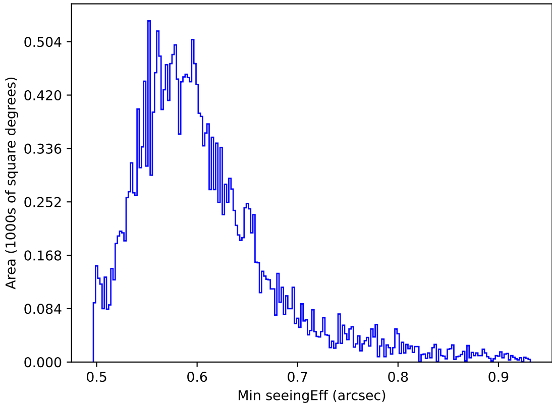
ddf_acor_sf10_lsf20_lsr10_v3.4_10yrs All sky all bands: Min seeingEff
