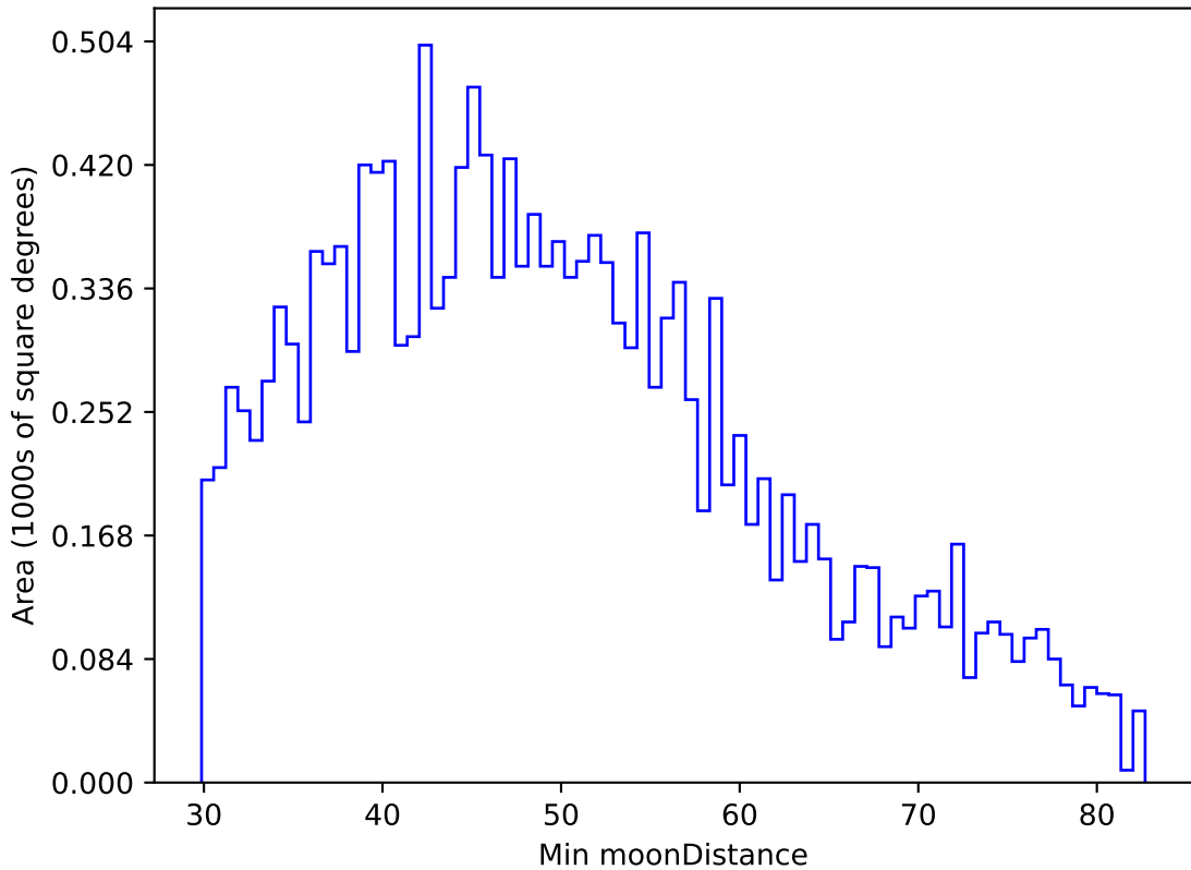
ddf_acor_sf10_lsf20_lsr10_v3.4_10yrs WFD u band: Min moonDistance
