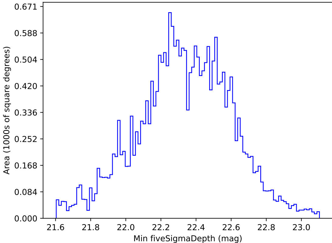
ddf_acor_sf10_lsf20_lsr10_v3.4_10yrs All sky u band: Min fiveSigmaDepth
