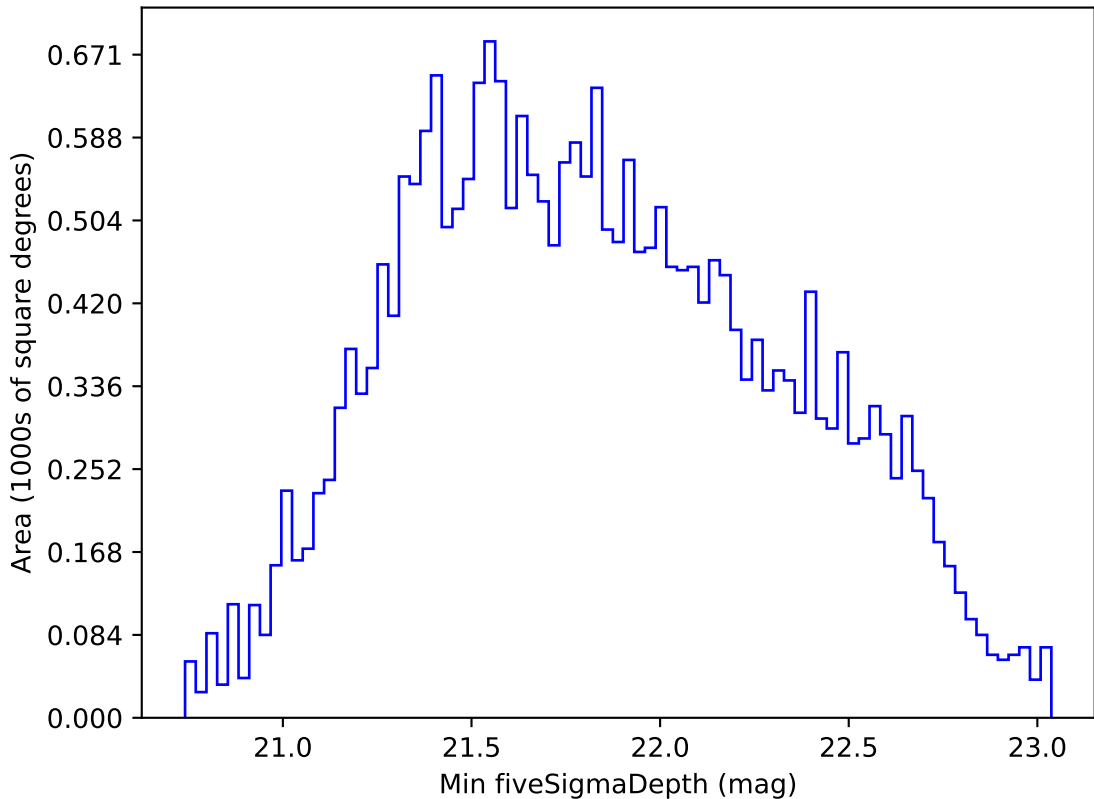
ddf_acor_sf10_lsf20_lsr10_v3.4_10yrs All sky i band: Min fiveSigmaDepth
