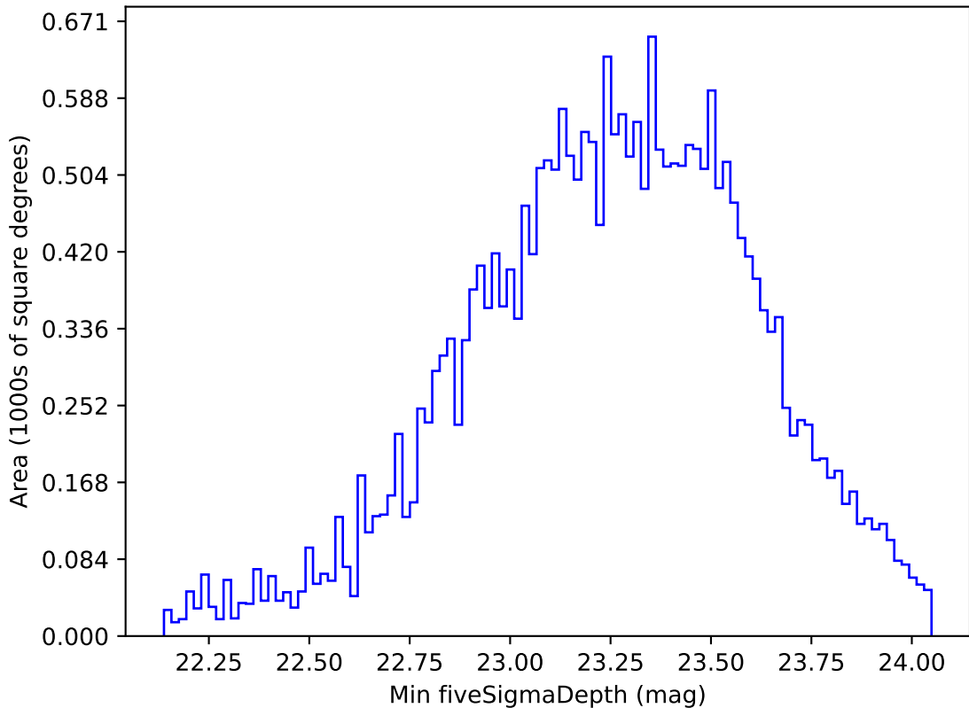
ddf_acor_sf10_lsf20_lsr10_v3.4_10yrs All sky g band: Min fiveSigmaDepth
