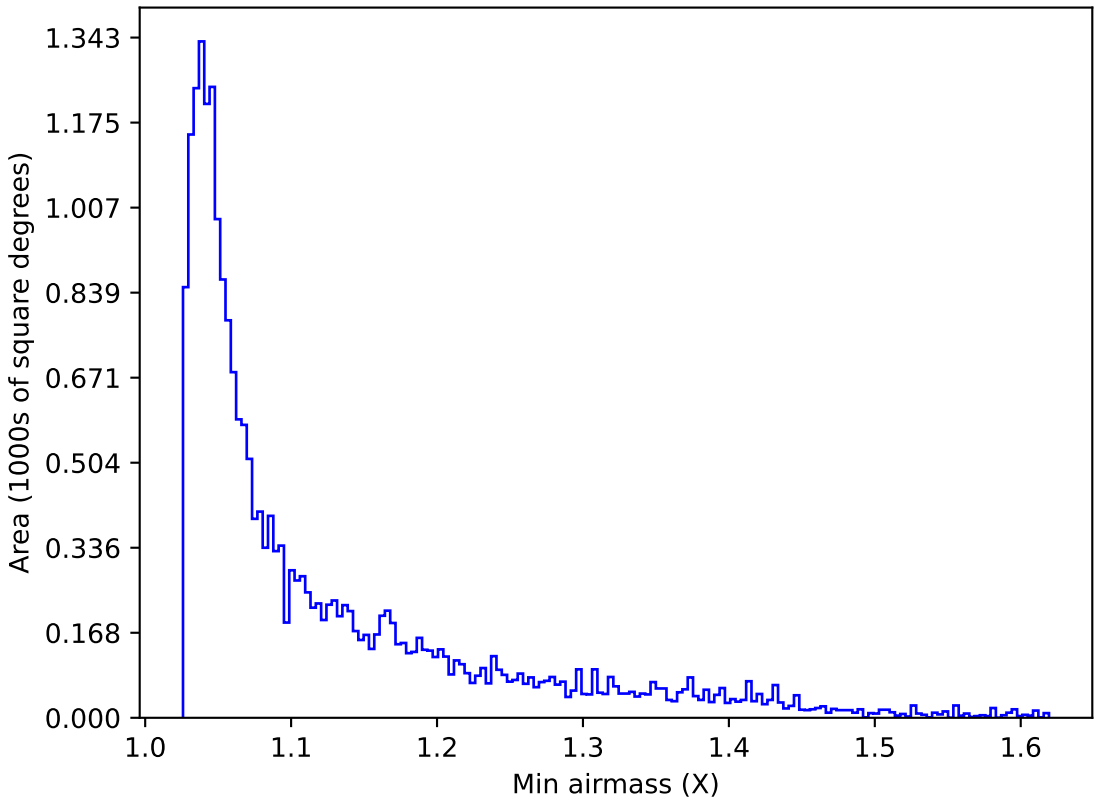
ddf_acor_sf10_lsf20_lsr10_v3.4_10yrs Yr 1 y band: Min airmass
