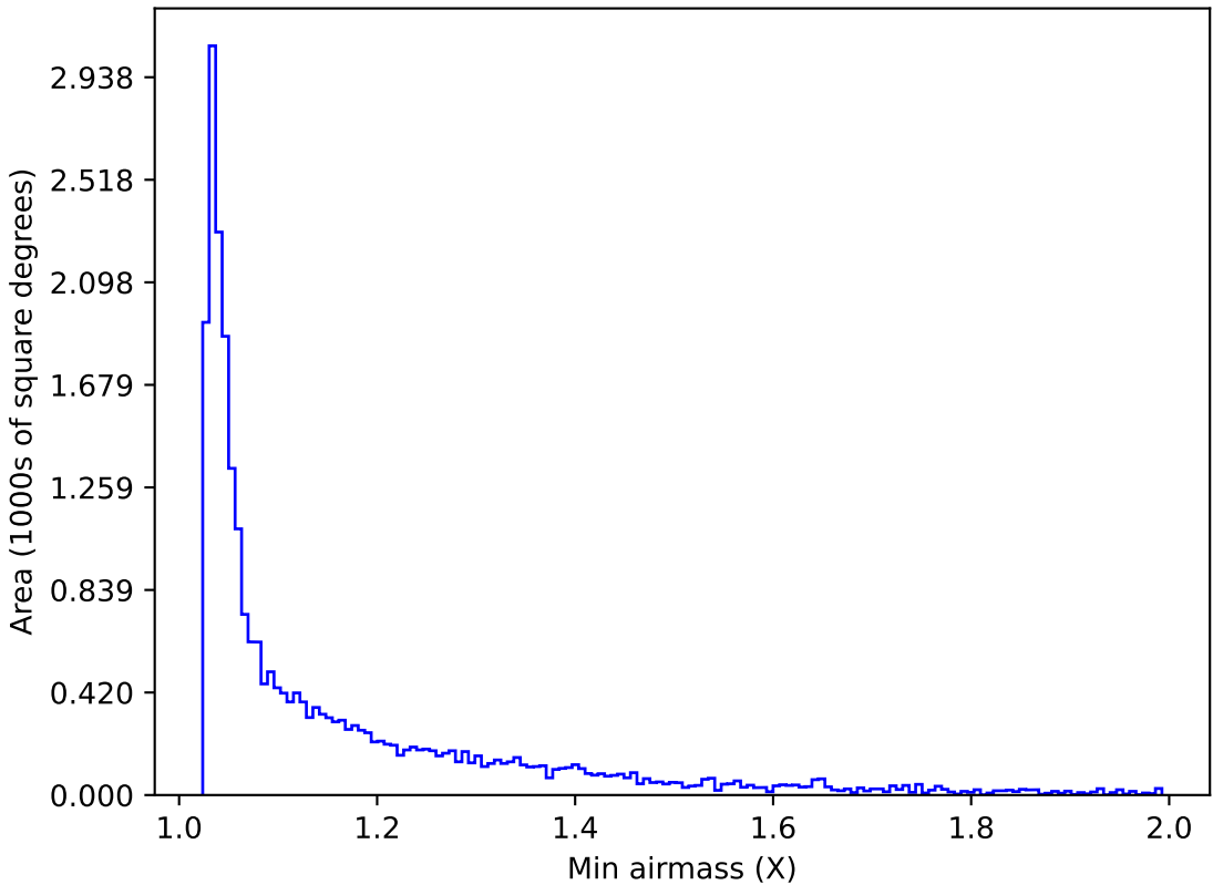
ddf_acor_sf10_lsf20_lsr10_v3.4_10yrs Yr 1 r band: Min airmass
