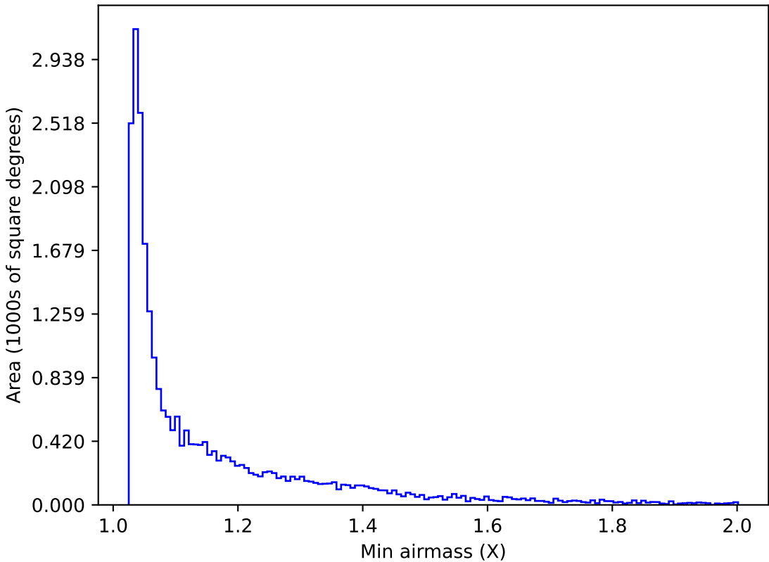
ddf_acor_sf10_lsf20_lsr10_v3.4_10yrs Yr 1 i band: Min airmass
