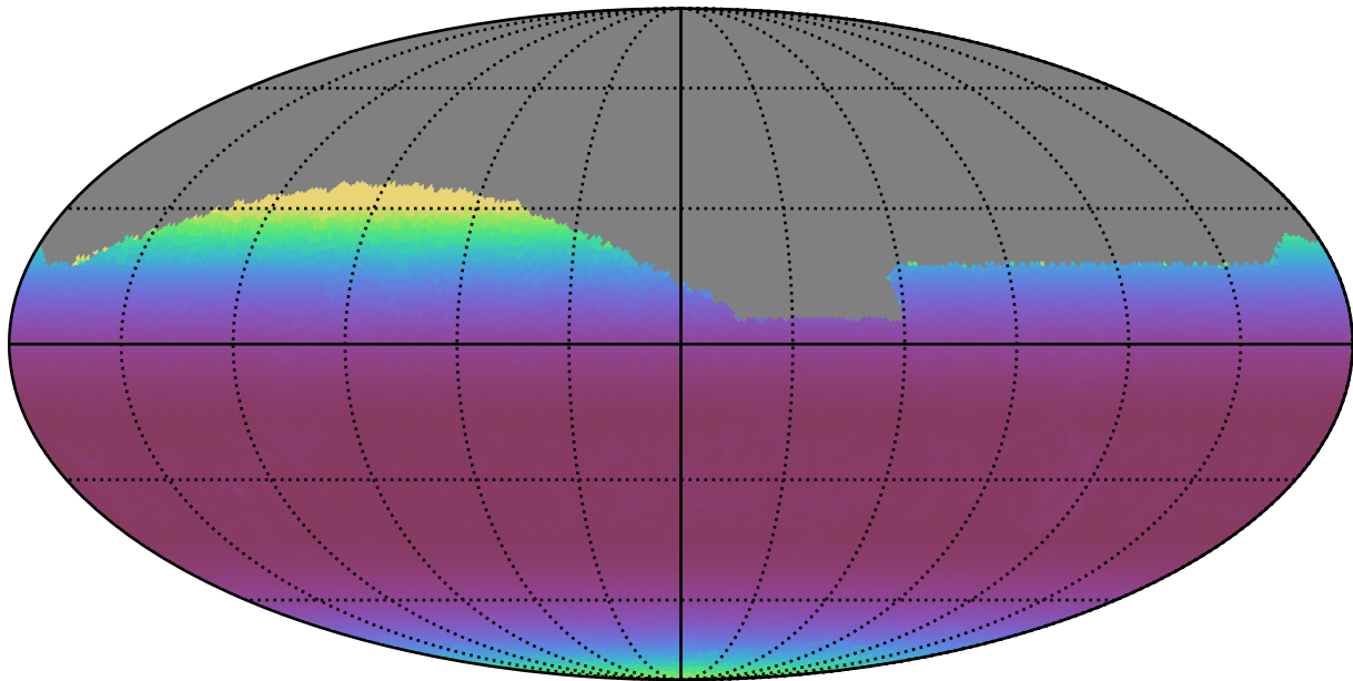
ddf_acor_sf10_lsf20_lsr10_v3.4_10yrs Yr 1 all bands: Min airmass
