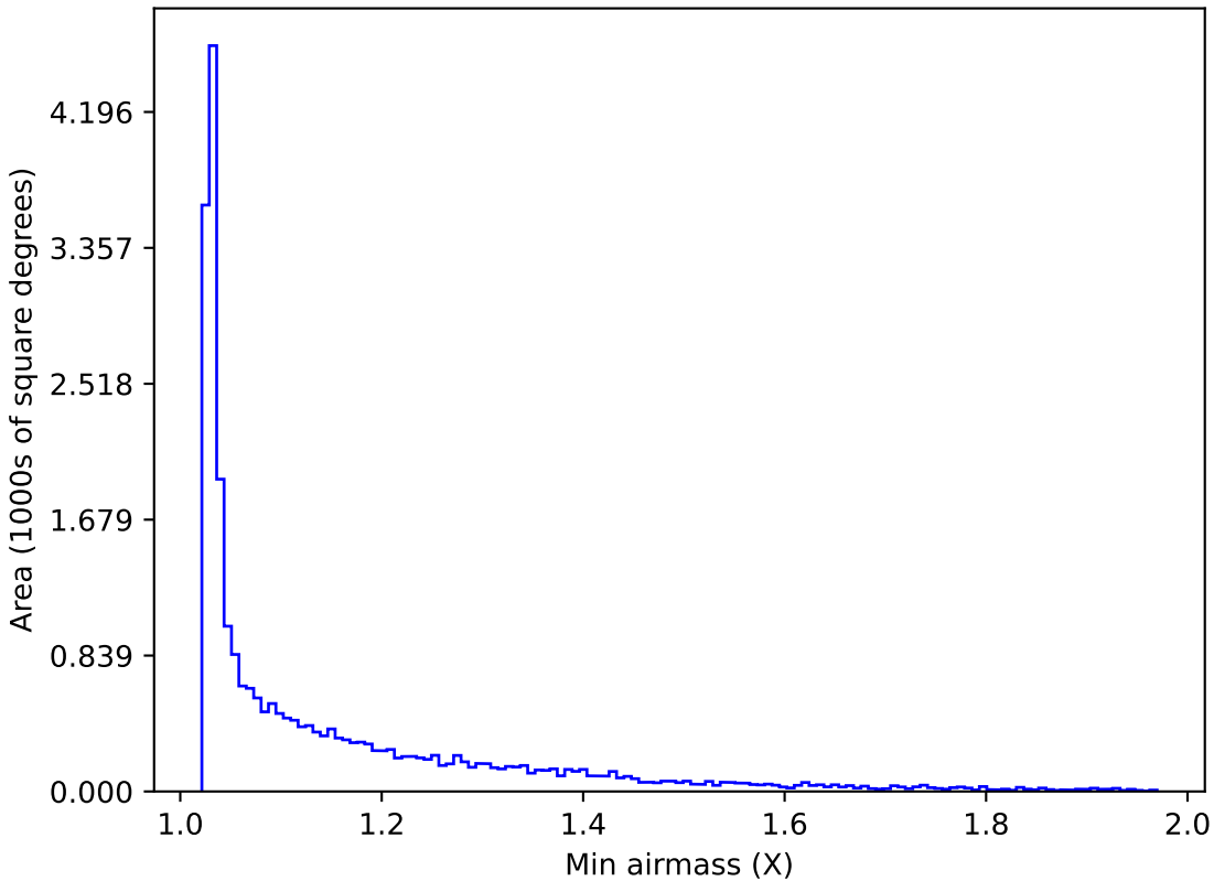
ddf_acor_sf10_lsf20_lsr10_v3.4_10yrs Yr 1 all bands: Min airmass
