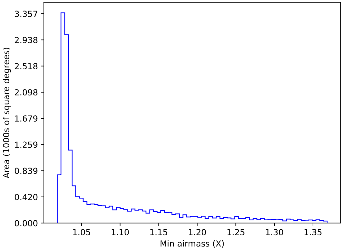
ddf_acor_sf10_lsf20_lsr10_v3.4_10yrs WFD z band: Min airmass
