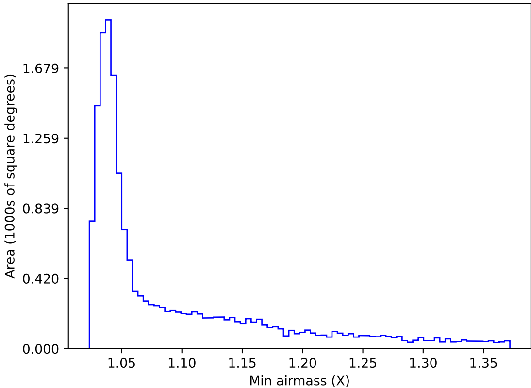
ddf_acor_sf10_lsf20_lsr10_v3.4_10yrs WFD u band: Min airmass
