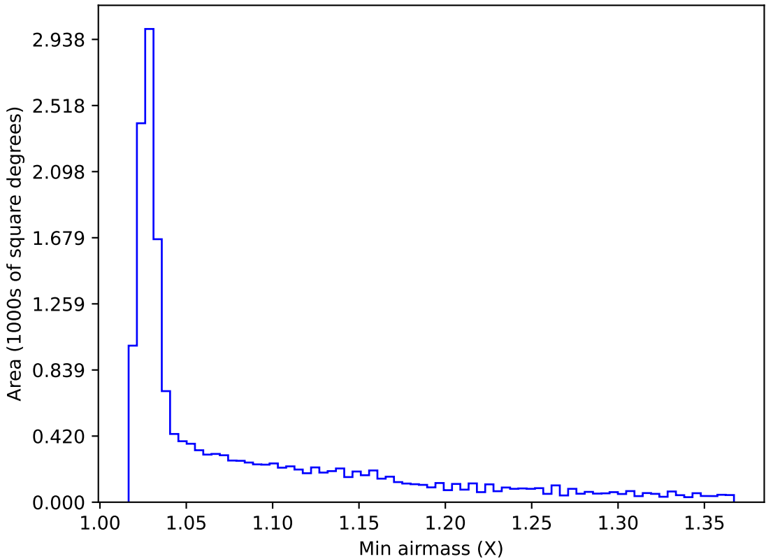
ddf_acor_sf10_lsf20_lsr10_v3.4_10yrs WFD r band: Min airmass
