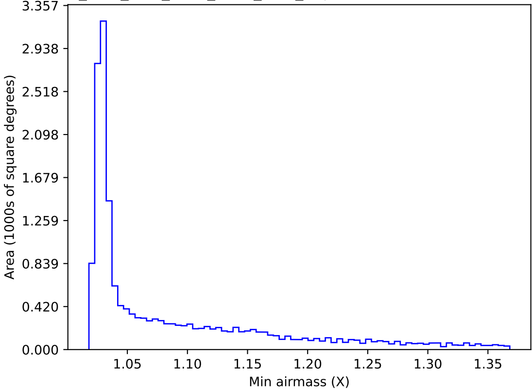
ddf_acor_sf10_lsf20_lsr10_v3.4_10yrs WFD i band: Min airmass
