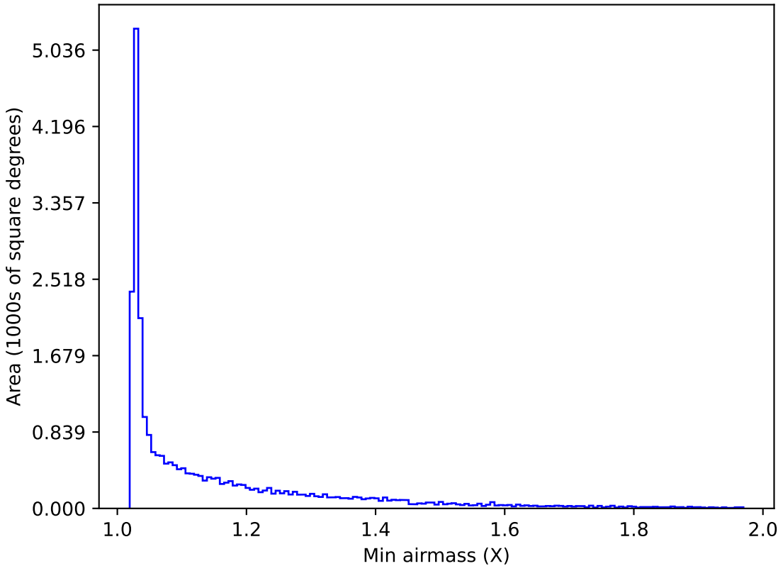
ddf_acor_sf10_lsf20_lsr10_v3.4_10yrs All sky z band: Min airmass
