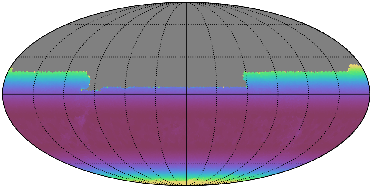
ddf_acor_sf10_lsf20_lsr10_v3.4_10yrs All sky y band: Min airmass
