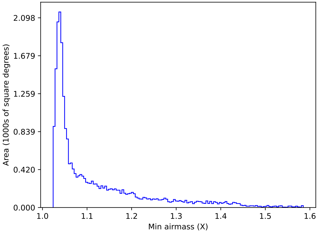
ddf_acor_sf10_lsf20_lsr10_v3.4_10yrs All sky u band: Min airmass
