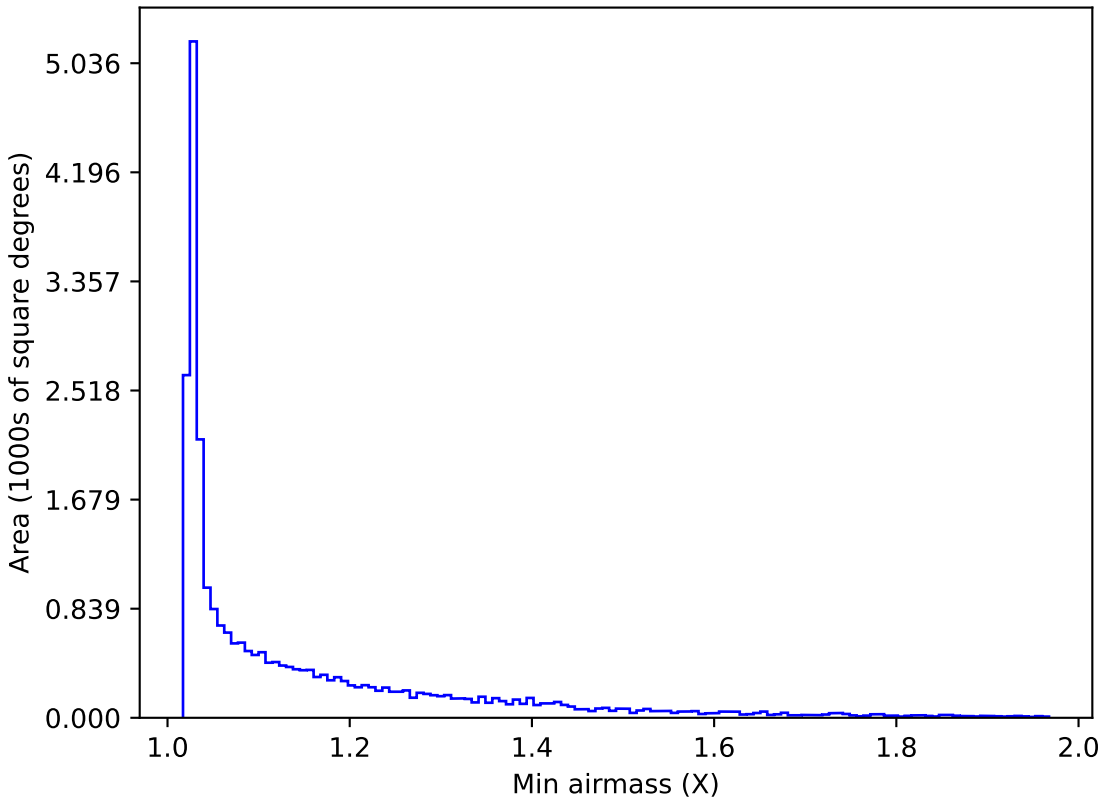
ddf_acor_sf10_lsf20_lsr10_v3.4_10yrs All sky r band: Min airmass
