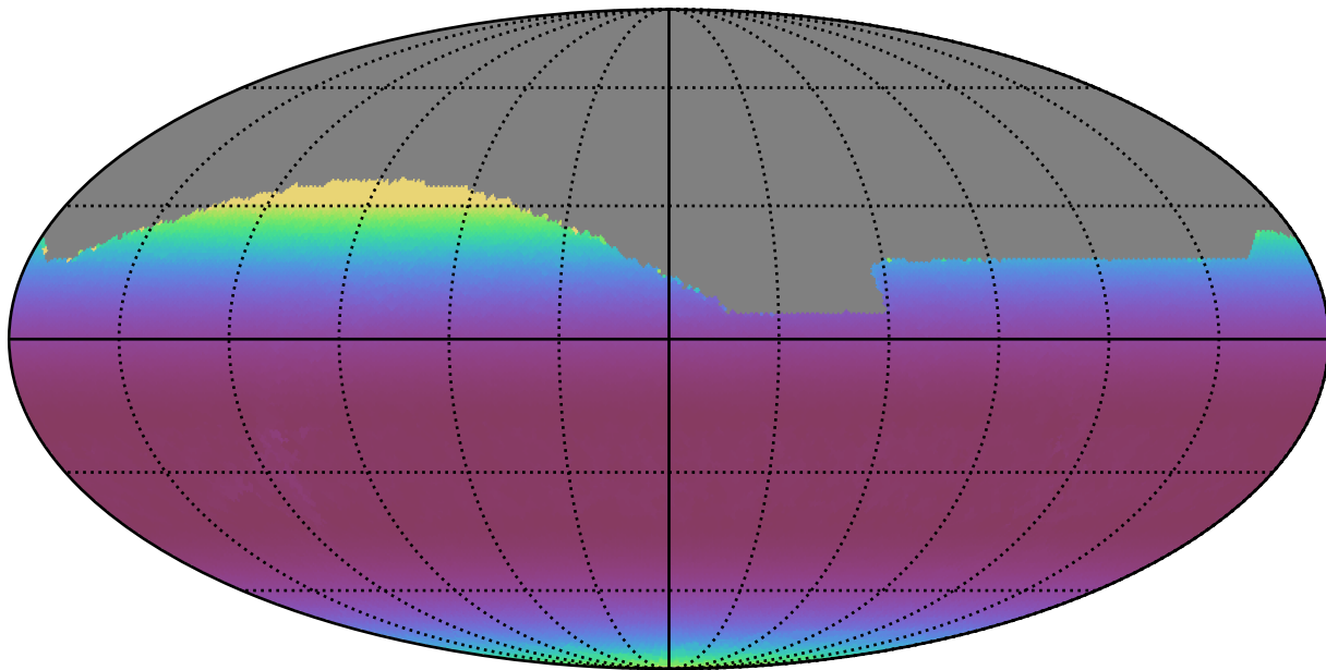
ddf_acor_sf10_lsf20_lsr10_v3.4_10yrs All sky i band: Min airmass
