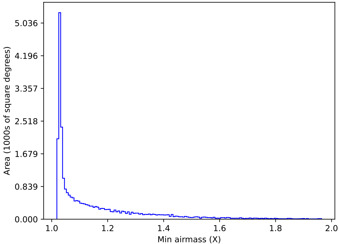
ddf_acor_sf10_lsf20_lsr10_v3.4_10yrs All sky i band: Min airmass
