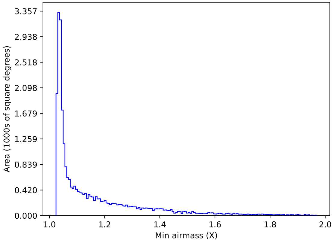
ddf_acor_sf10_lsf20_lsr10_v3.4_10yrs All sky g band: Min airmass
