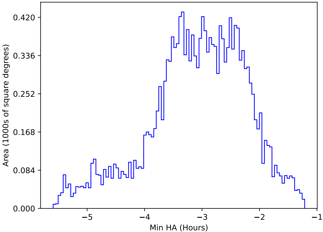
ddf_acor_sf10_lsf20_lsr10_v3.4_10yrs WFD u band: Min HA
