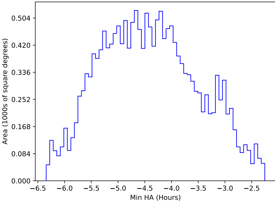
ddf_acor_sf10_lsf20_lsr10_v3.4_10yrs WFD r band: Min HA
