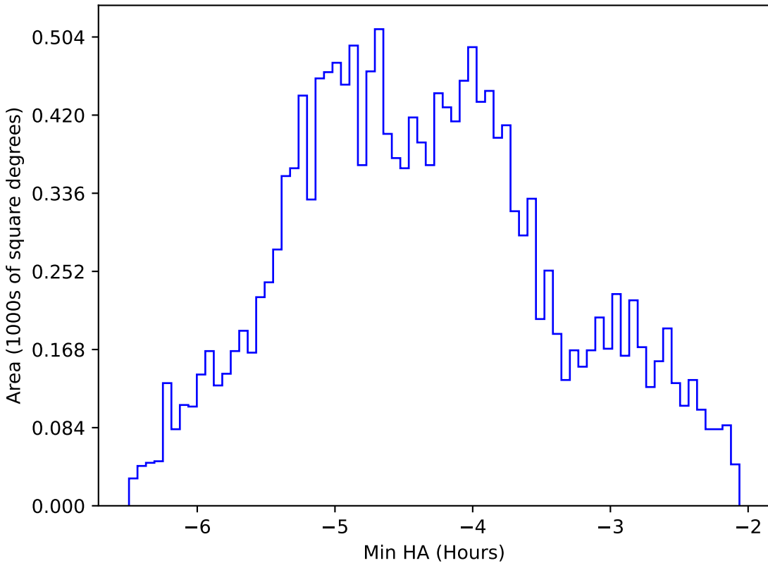
ddf_acor_sf10_lsf20_lsr10_v3.4_10yrs WFD i band: Min HA
