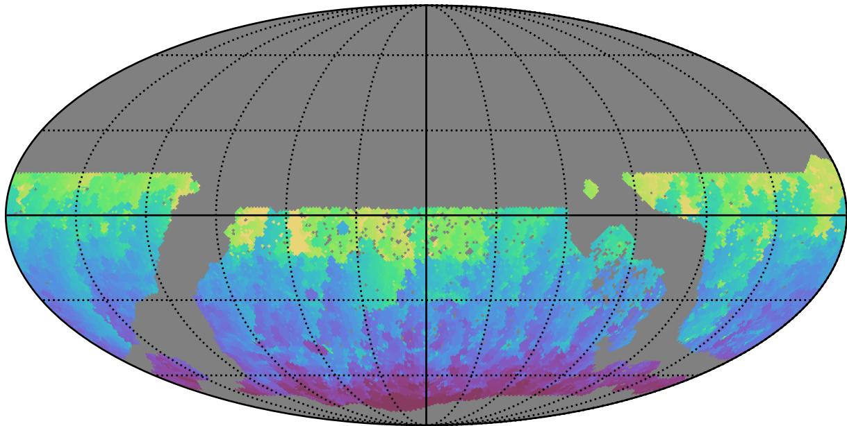
ddf_acor_sf10_lsf20_lsr10_v3.4_10yrs WFD g band: Min HA
