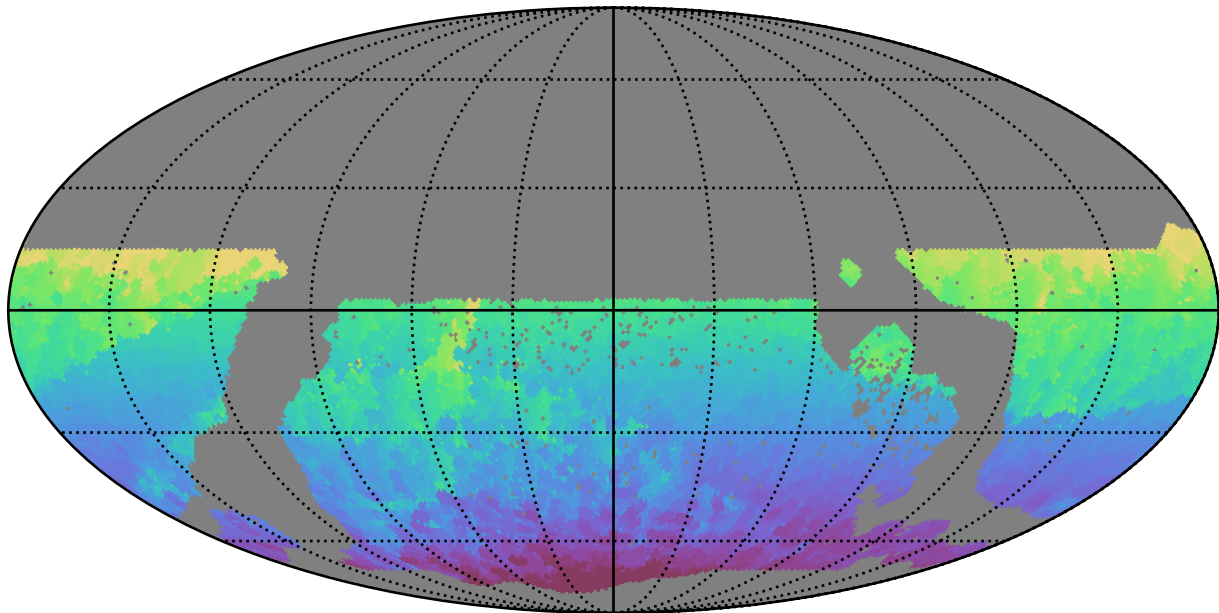
ddf_acor_sf10_lsf20_lsr10_v3.4_10yrs WFD all bands: Min HA
