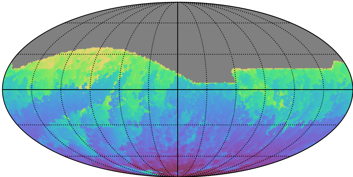
ddf_acor_sf10_lsf20_lsr10_v3.4_10yrs All sky z band: Min HA
