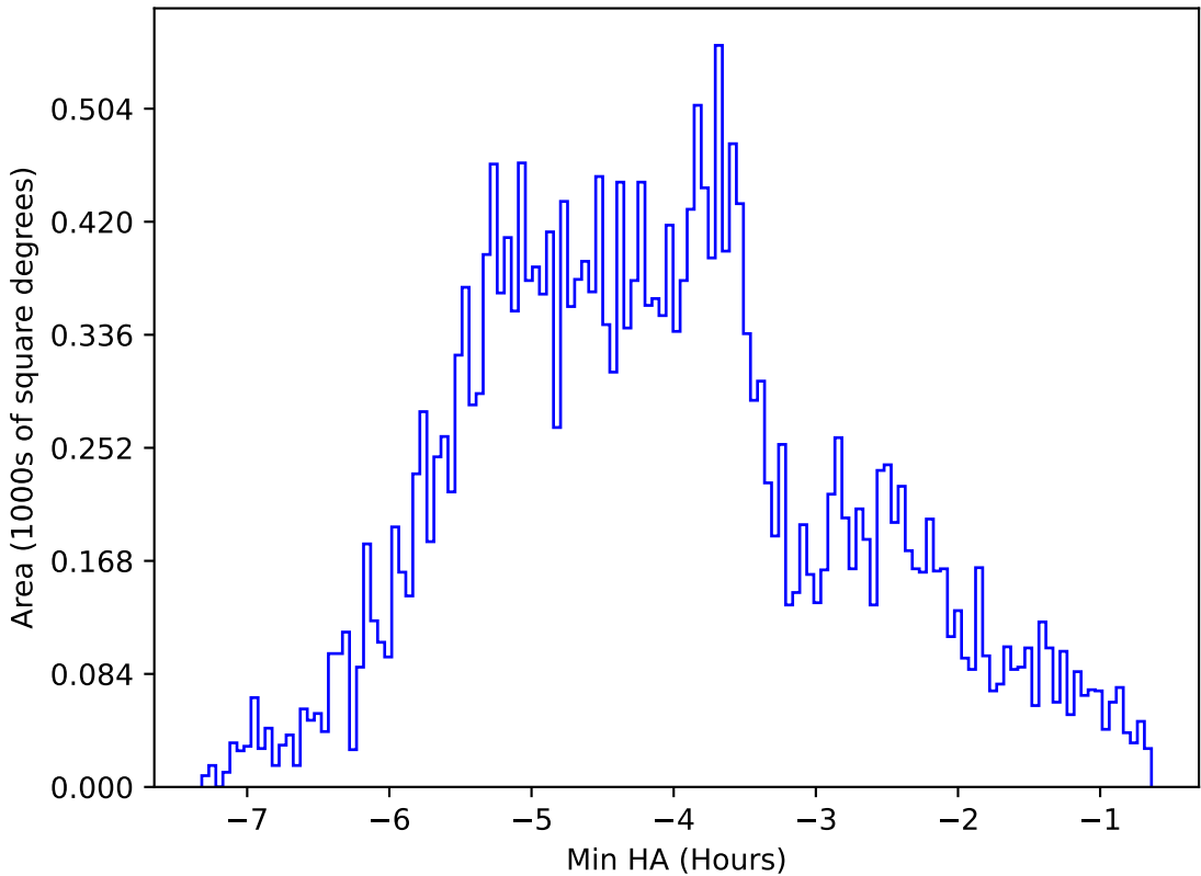
ddf_acor_sf10_lsf20_lsr10_v3.4_10yrs All sky z band: Min HA
