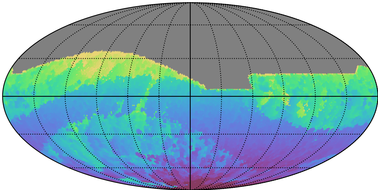
ddf_acor_sf10_lsf20_lsr10_v3.4_10yrs All sky r band: Min HA
