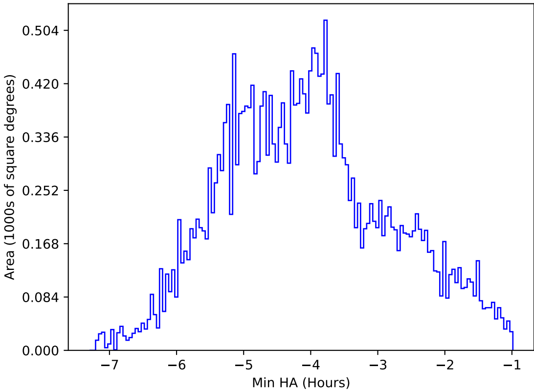
ddf_acor_sf10_ls20_lsr10_v3.4_10yrs All sky i band: Min HA
