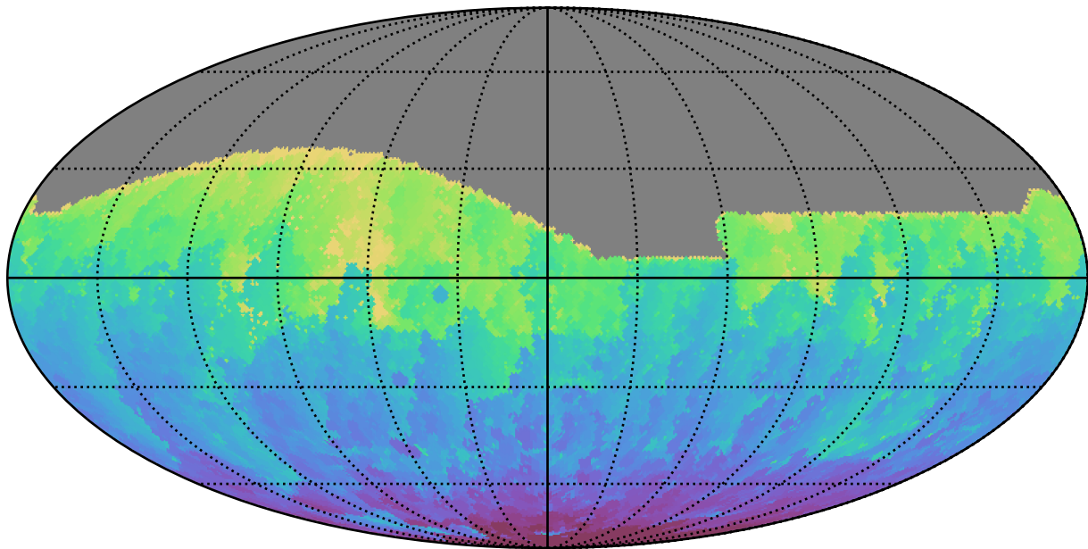
ddf_acor_sf10_lsf20_lsr10_v3.4_10yrs All sky g band: Min HA
